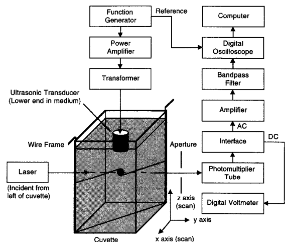
Fig. 1. Setup of imaging of turbid media using ultrasound-modulated scattered laser light. The arrows between blocks represent electrical signals, and the arrows from the laser and from the cuvette represent optical signals.
