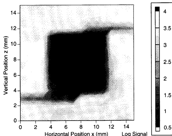
Fig. 2. Two-dimensional image of a buried glass cube plotted on a logarithmic scale of the peak-to-peak voltage signals of the ultrasound-modulated light in millivolts. The holding wire on the top right and bottom left of the cube was observed at the same time.
