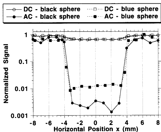
Fig. 3. One-dimensional images of a black and a blue glass sphere obtained with the dc unmodulated laser-light signals and the ac ultrasound-modulated laser-light signals.
